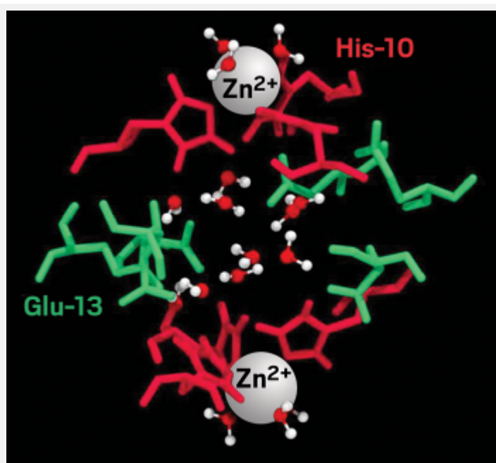
Two zinc cations and ten water molecules stabilize the interior cavity of the insulin hexamer.
