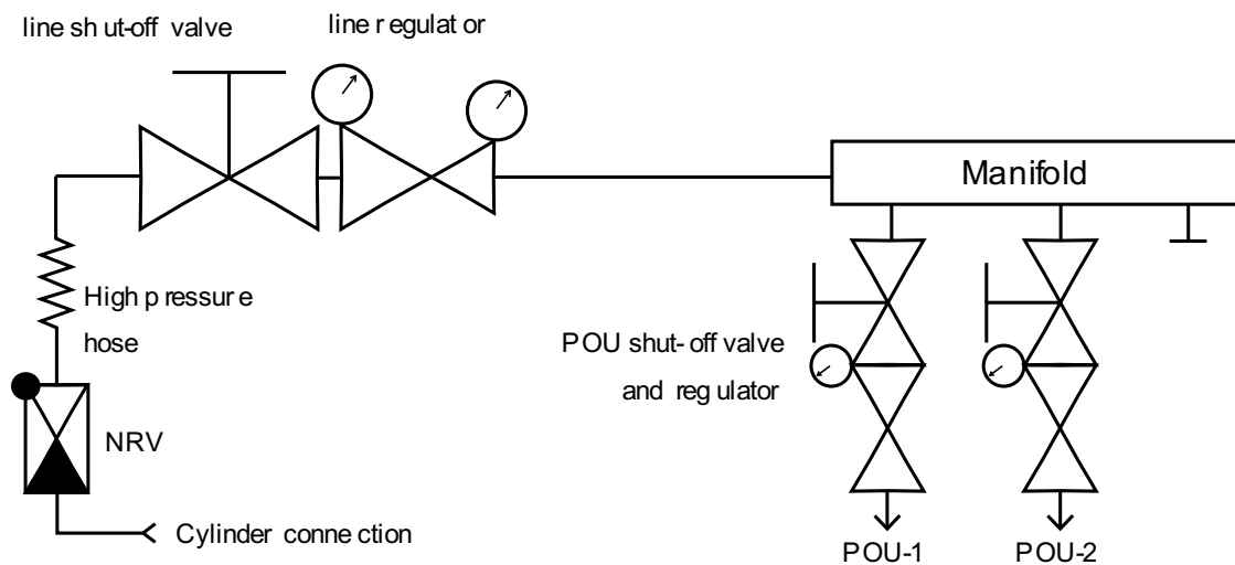
Figure 2: Sample gas line configuration
