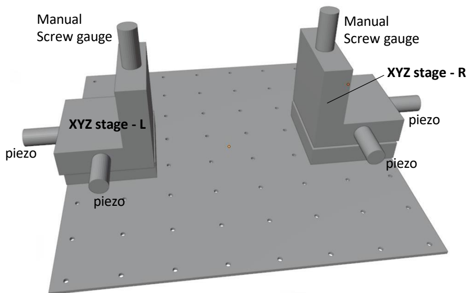
Figure 1 : Illustration of XYZ piezo actuated linear stage setup. Image NOT to scale
